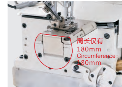
超细嘴180mm，缝制范围广 180mm small cylinder bed, wide range of application
