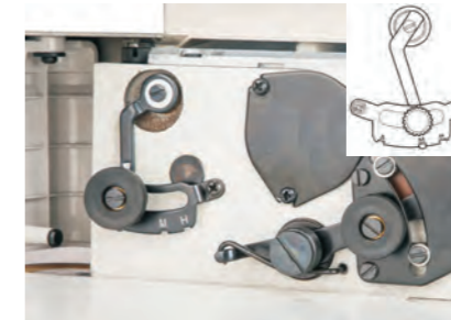
薄厚随意可调，适应范围更广 Thickness adjustable freely, wider range of adaptation
