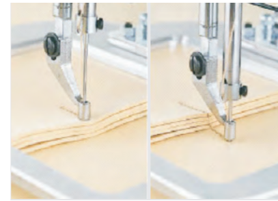
智能中压脚 Intelligent central presser foot
