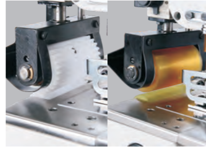
可选配后拖轮，缝薄过厚皆适宜 Optional puller, capable for light to heavy material
