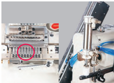
Auto thread trimming, auto presser foot lifter
