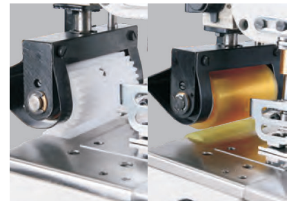
Optional puller, capable for light to heavy material
