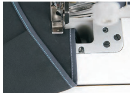
One machine with fabric edge cutter and tape binder functions
